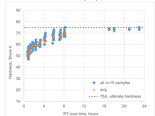
Hardness Build Profile, ASTM D2240 with operating stand 3"x6" cylinders, gravel loaded to within 1/2" from top Ambient 72°F (22°C) cure
